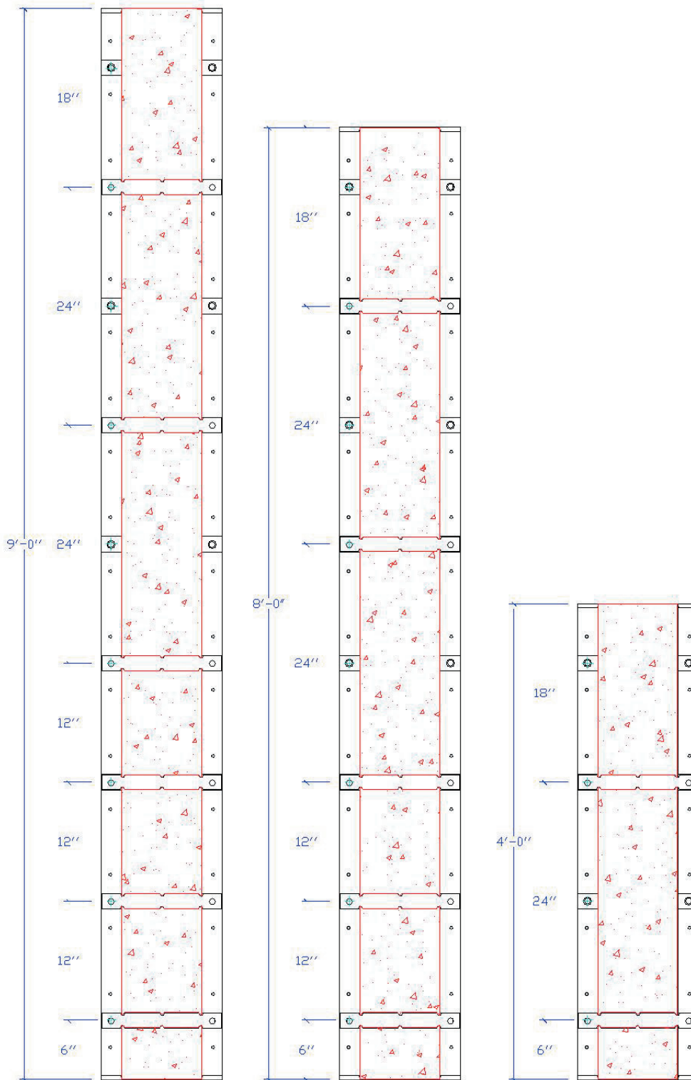
6•12 Hole Pattern
